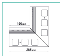
K40 90 INTERNAL CORNER
