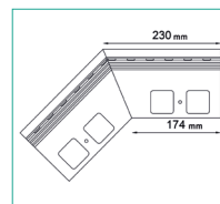
K40 135 EXTERNAL CORNER
