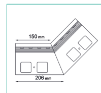
K40 135 INTERNAL CORNER
