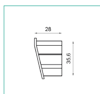
OPK30/OPK40 R+L WALL PROTECTION END CAPS
