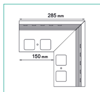
K40 90 EXTERNAL CORNER
