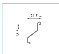
LK30/LK40 DRIP EDGE CLIP
