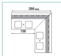
K30 90 EXTERNAL CORNER
