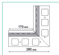
K30 90 INTERNAL CORNER
