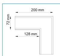
RK65 90 INTERNAL GUTTER ANGLE
