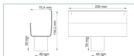
RK65 RUNNING OUTLET
