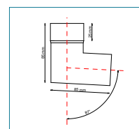
RK65 87 DOWNPIPE OFFSET BEND
