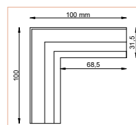
K20/K20R RETURN PIECES
