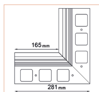
K20R 90 INTERNAL CORNER
