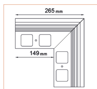
K20R 90 EXTERNAL CORNER
