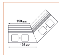
K20 135 INTERNAL CORNER
