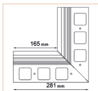
K20 90 INTERNAL CORNER
