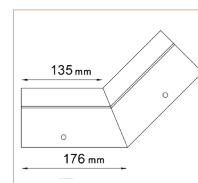
K10 135 INTERNAL CORNER
