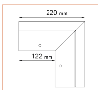
K10 90 EXTERNAL CORNER
