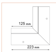
K10 90 INTERNAL CORNER
